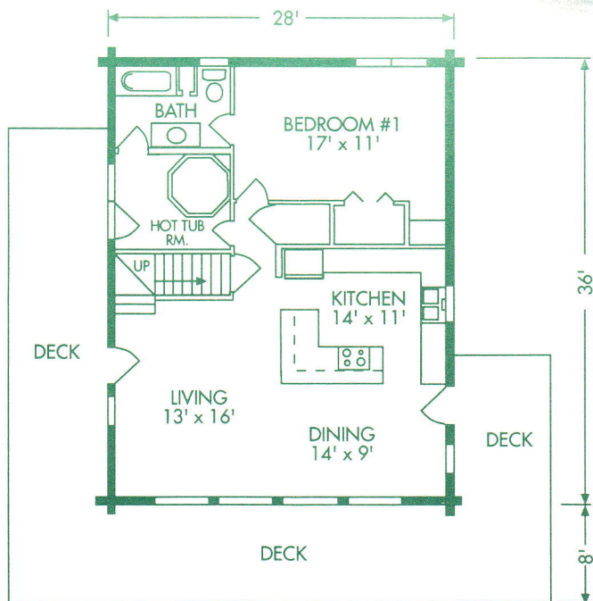
MAIN FLOOR
