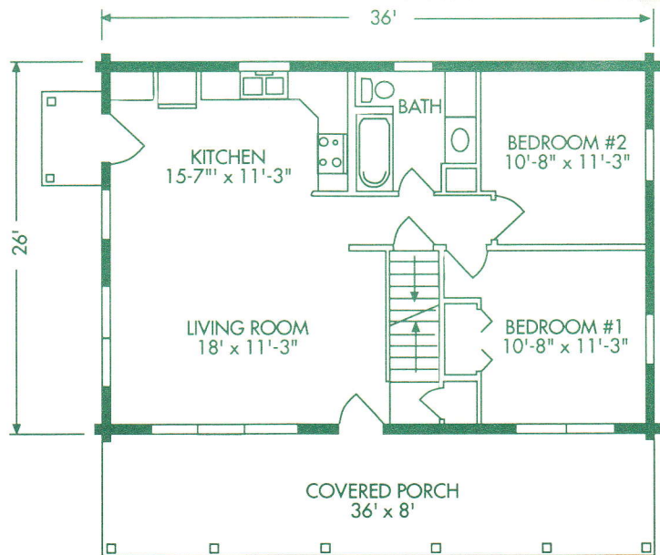
MAIN FLOOR
